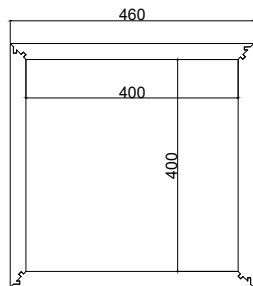
VISTA SUPERIOR S/ TAMPA
